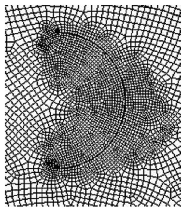
Fig. 3. Detail of mesh around the blade surface
