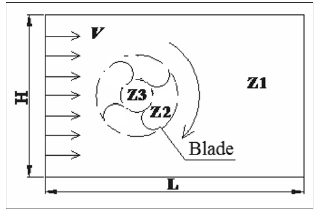
Fig. 2. Simulation model of a 4-blade VAWT
