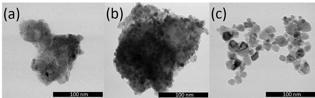
Fig. 3. TEM images of BaTiO 3 perovskites synthesized in the (a) Si 3 N 4 , (b) FeNi and (c) TC grinding vessels
