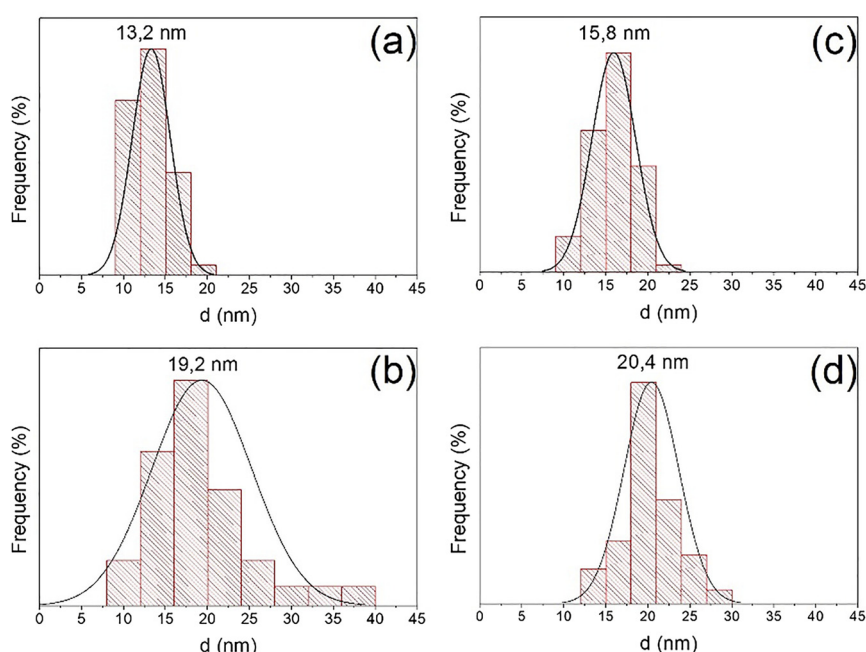
Fig. 5. Histograms of the particle size distribution of \text{BaTiO}_3 (a, b) and \text{ZnTiO}_3 (c, d) perovskites produced in the FeNi (a, c) and TC (b, d) grinding vessels
