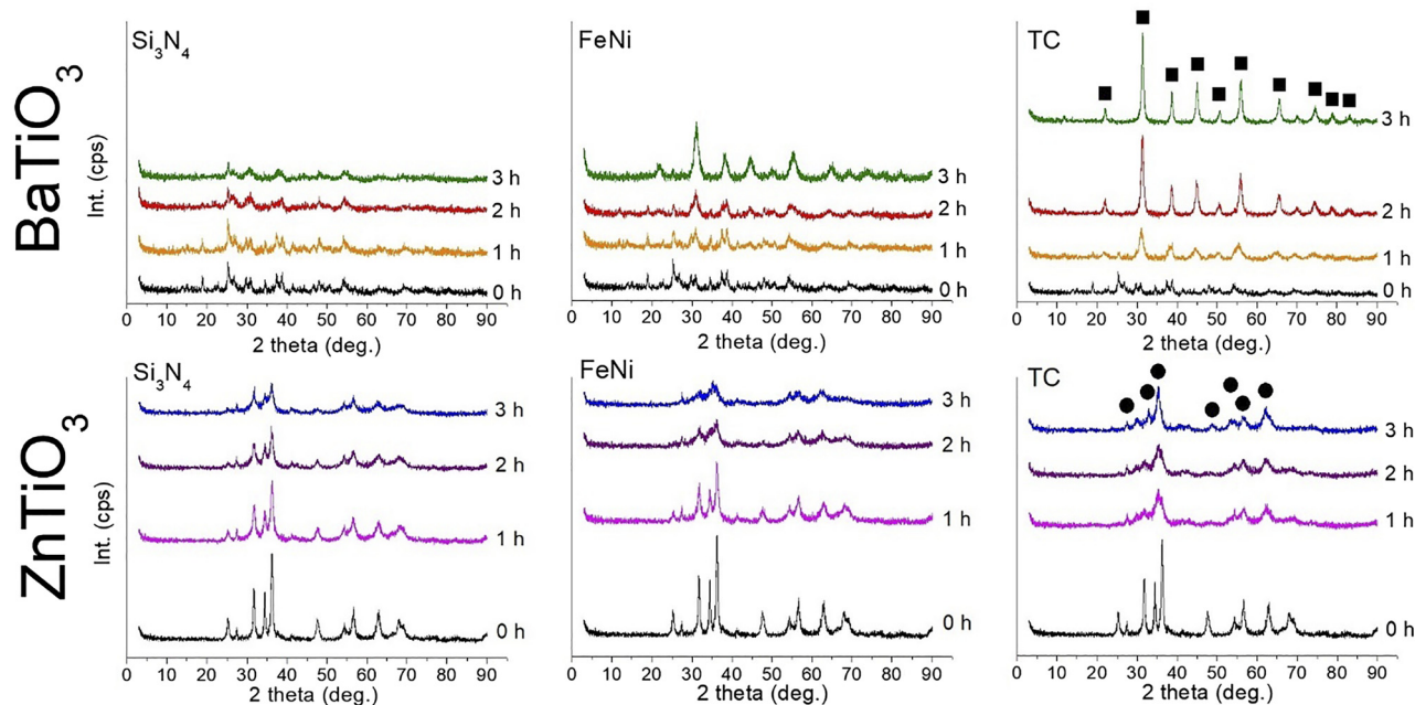
Fig. 2. Results of XRD measurements. The 0-h sample means the BaO/ZnO-TiO 2 starting materials mixture. ■ typical reflections of BaTiO 3 perovskite. ● typical reflections of ZnTiO 3 perovskite
