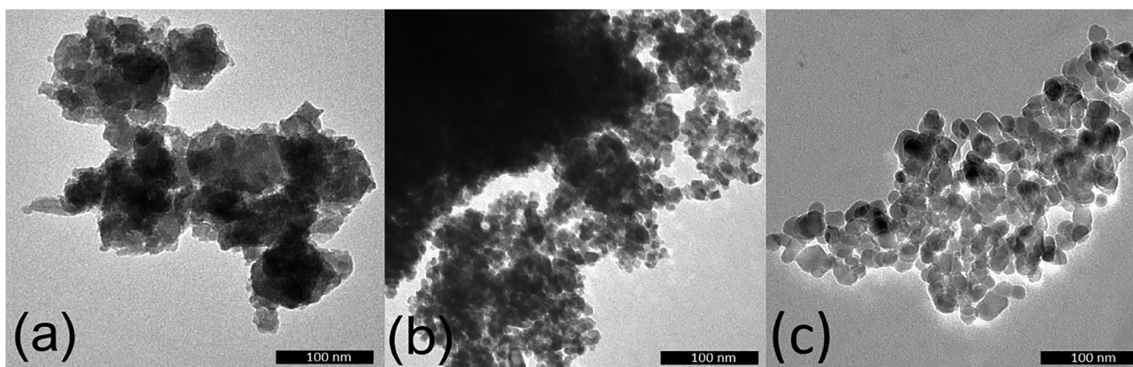
Fig. 4. TEM images of \text{ZnTiO}_3 perovskites synthesized in the (a) \text{Si}_3\text{N}_4 , (b) FeNi and (c) TC grinding vessels
