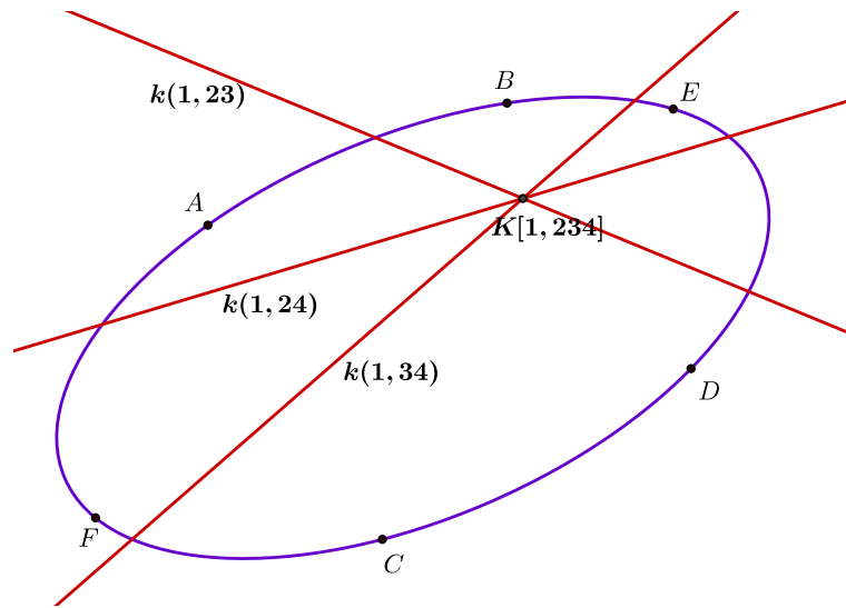
FIGURE 3. The Pascals k(1, 23) , k(1, 24) , k(1, 34) concur at the Kirkman point K[1, 234] .
