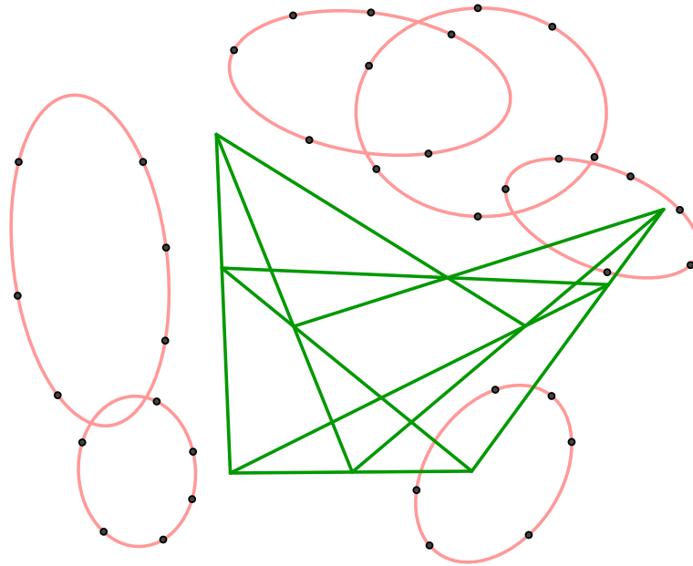
FIGURE 5. Conical sextuples associated to a Desargues configuration
