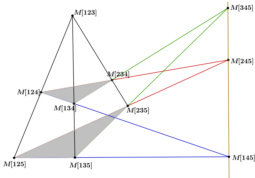
FIGURE 1. Desargues configuration. The line labels are omitted in order to avoid clutter.
