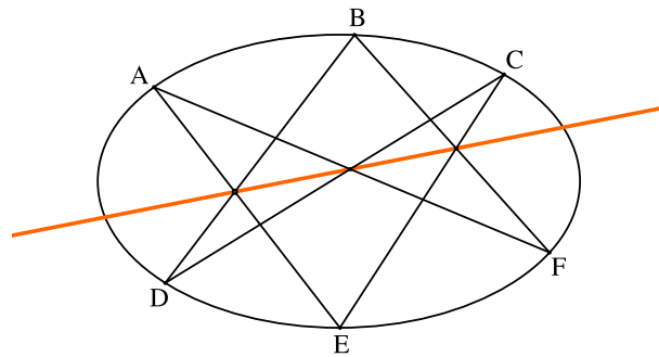
FIGURE 2. Pascal's theorem
