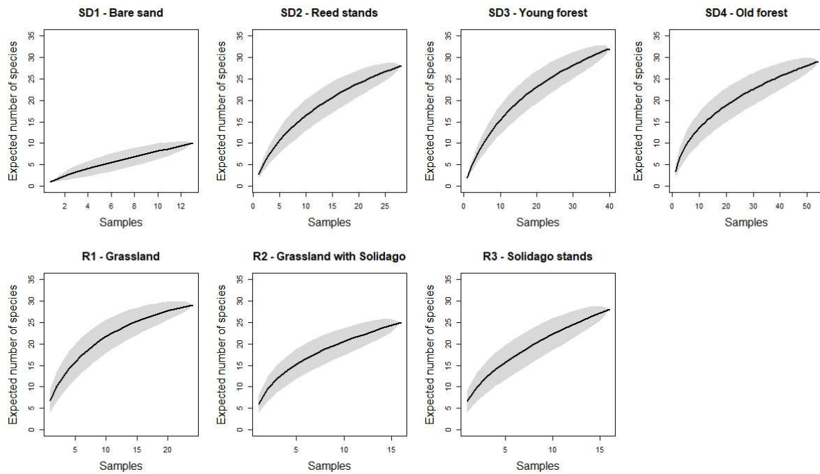
Figure A1. Estimations of carabid species richness according to Chao estimators (with 95% confidence intervals) in sludge deposits (upper line) and reclaimed area (bottom line).
